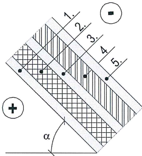
Figure 1. Roof construction design
